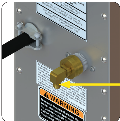
Plumbing Hook-Up
