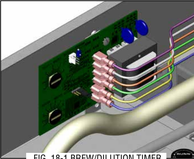
FIG. 18-1 BREW/DILUTION TIMER
